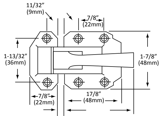
HEAVY DUTY MODEL NO. M15-9211
