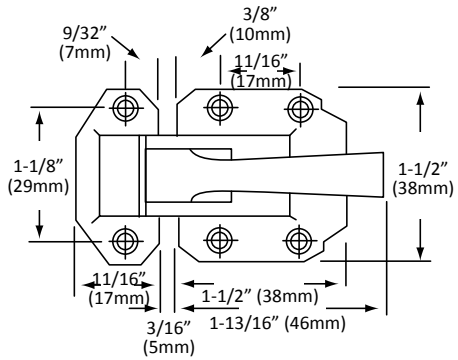
STANDARD DUTY MODEL NO. M15-9210
